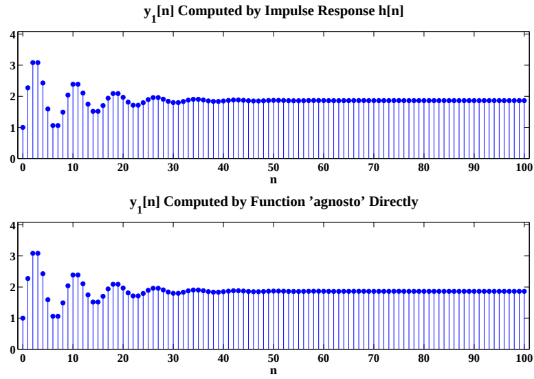
FIGURE 2.59: System response y_1[n] of input x_1[n] = u[n] .
