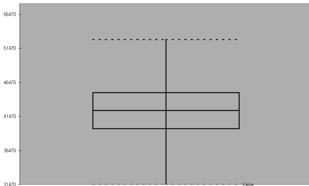
Box-and-whisker Plot
