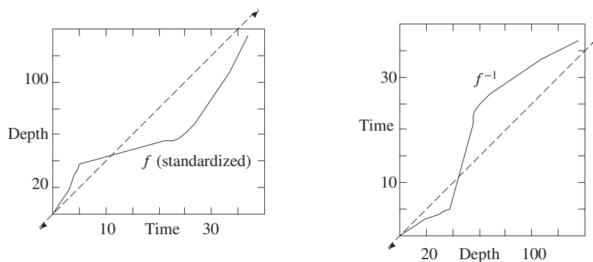
Figure 1.37: Graph of f , reflected to give that of f^{-1}
