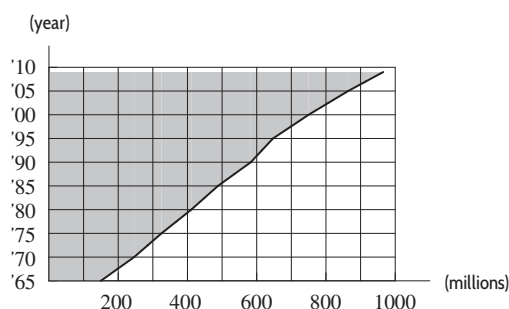
Figure 1.36: Graph of f^{-1}
