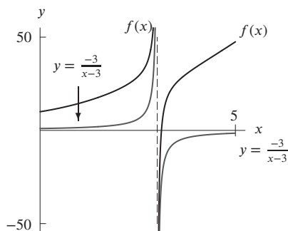
Figure 1.163: Close-up view of f(x) and y = -3/(x - 3)
