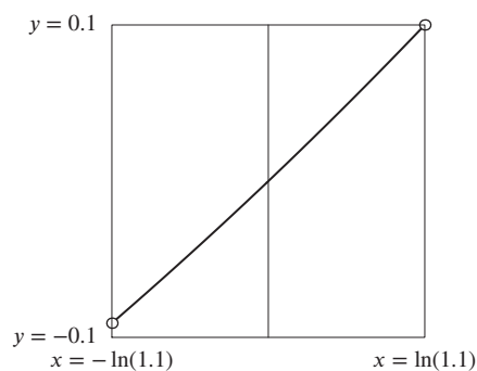
Figure 1.118: Graph of e^x - 1 with -\ln(1.1) < x < \ln(1.1)
