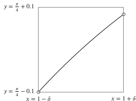
Figure 1.120: Graph of \arctan x with
