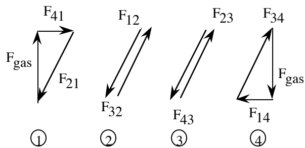
Force Diagrams
