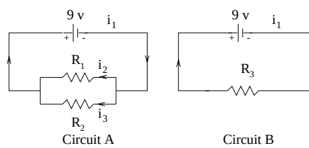
Figure 1.5 Exercise 1.3 assumed flows.
