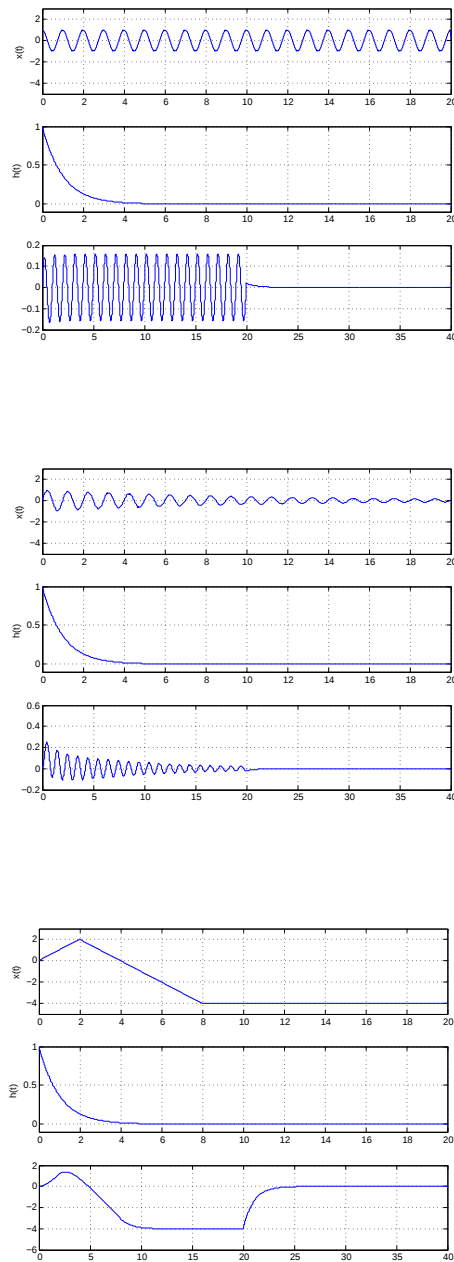
Figure 2.15: Problem 25: input, impulse response and output of convolution integral.
