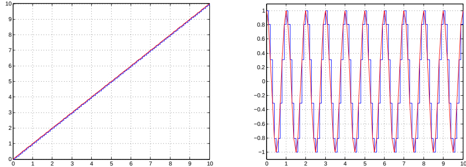
Figure 1.15: Problem 23: ‘Digitized’ ramp and cosine signals using ‘stairway to stars’
