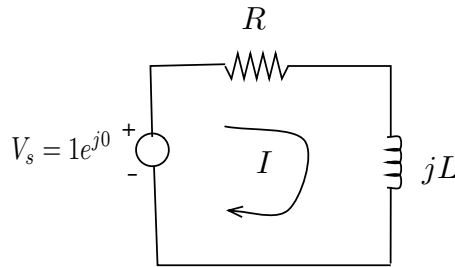
Figure 1.4: Problem 7: Phasor circuit.
