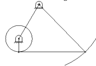
Crank-rocker linkage
