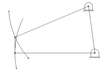
Double-rocker linkage.
