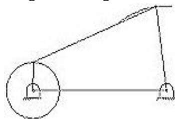
Crank-rocker linkage
