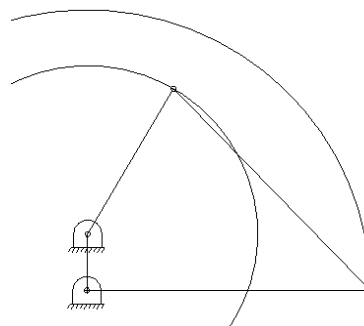
Drag-link linkage
