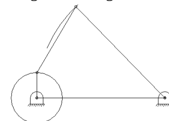
Crank-rocker linkage
