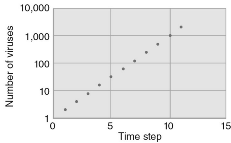
(b) Number of viruses versus time step (log plot)
