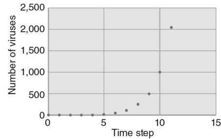
(a) Number of viruses versus time step
