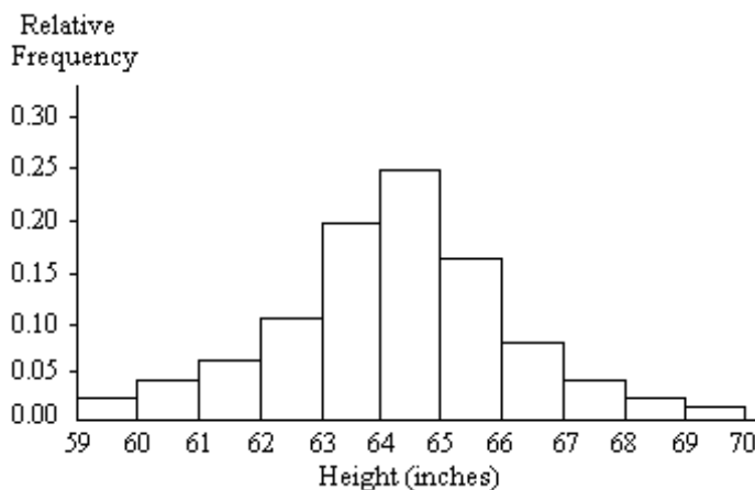
Histogram II
